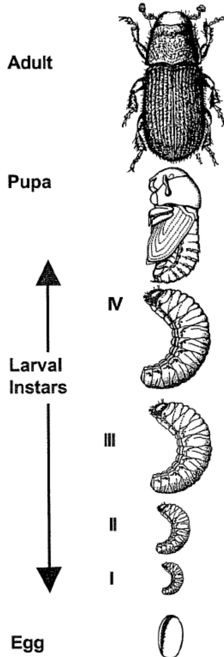
Figure 1. Bark beetle life cycle Redrawn from figures provided by Canadian Forestry Service
