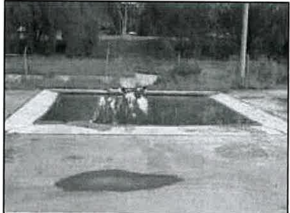
Figure 117. Vehicle and equipment wash area (CALTRANS 2003).
