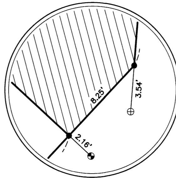
DETAIL M NOT TO SCALE
